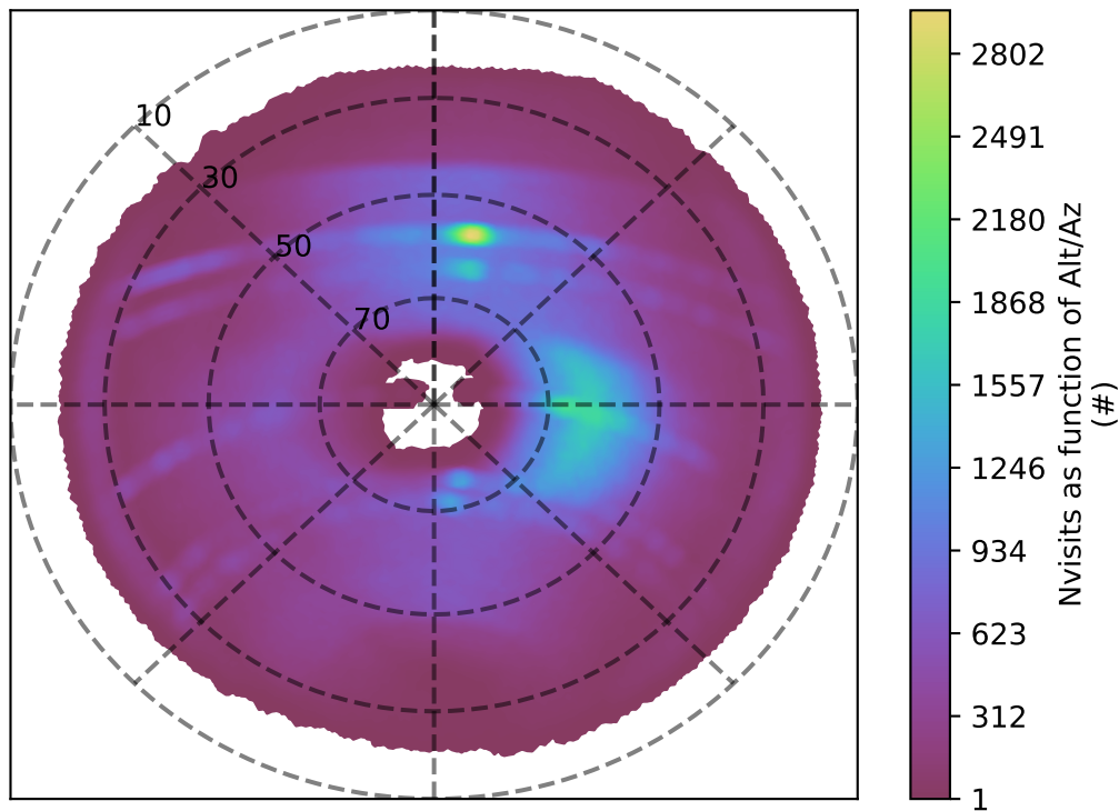
baseline_v3.5_10yrs r band: Nvisits as function of Alt/Az
