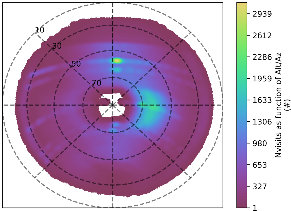
baseline_v3.5_10yrs i band: Nvisits as function of Alt/Az
