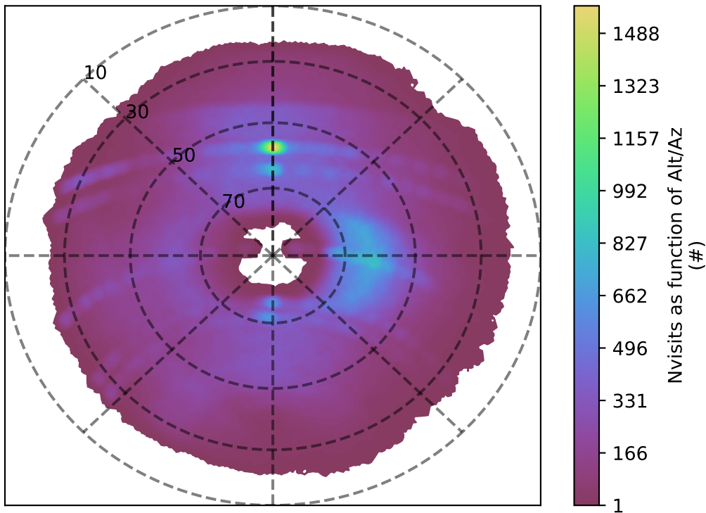
baseline_v3.5_10yrs g band: Nvisits as function of Alt/Az
