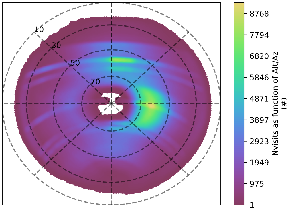
baseline_v3.5_10yrs all bands: Nvisits as function of Alt/Az
