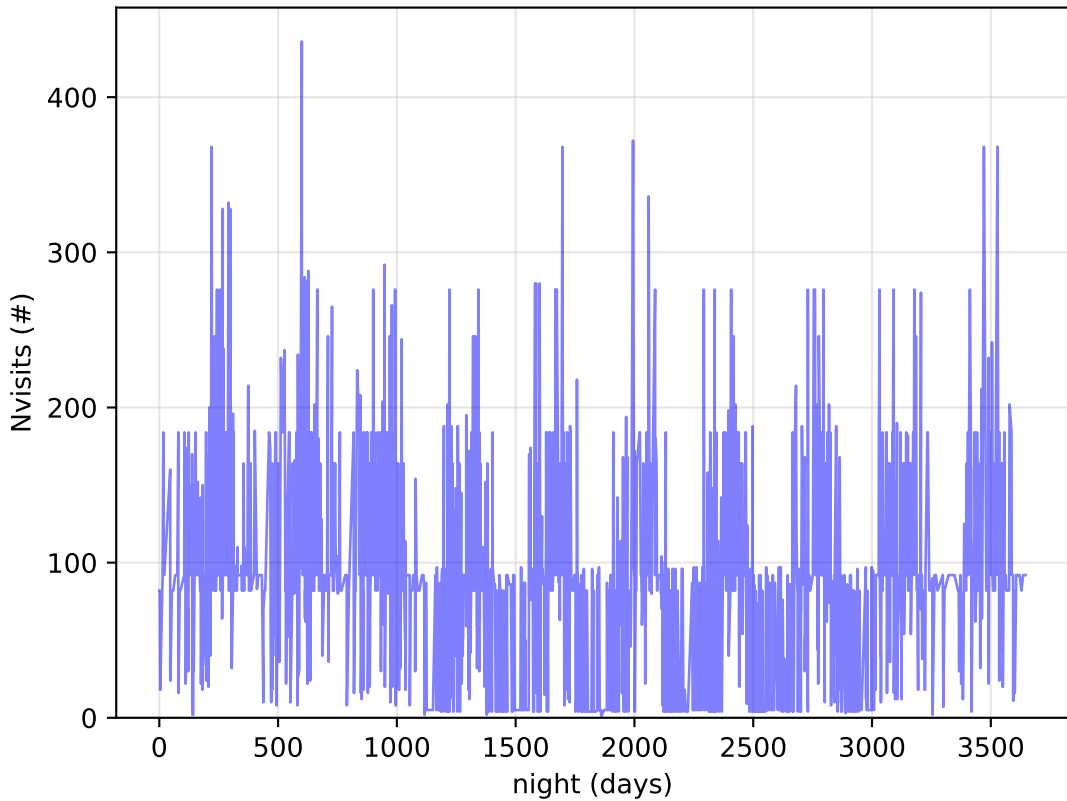
baseline_v3.5_10yrs DDF: Nvisits
