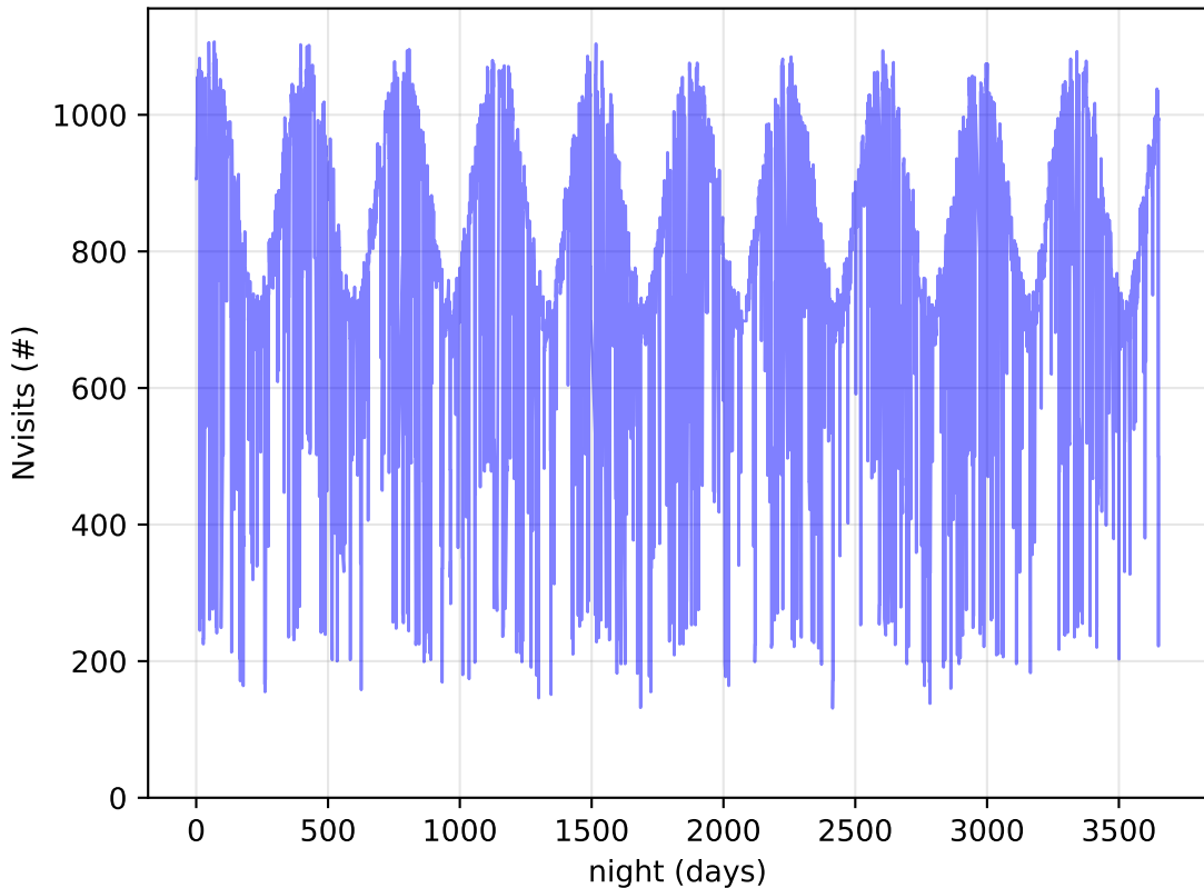
baseline_v3.5_10yrs All visits: Nvisits
