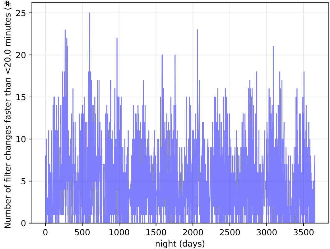
baseline_v3.5_10yrs Per Night: Number of filter changes faster than <20.0 minutes
