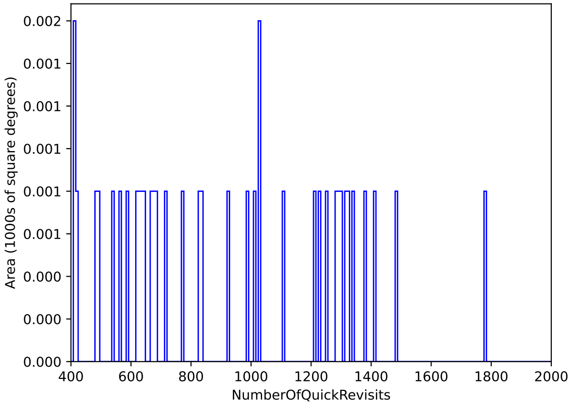
baseline_v3.5_10yrs WFD: NumberOfQuickRevisits
