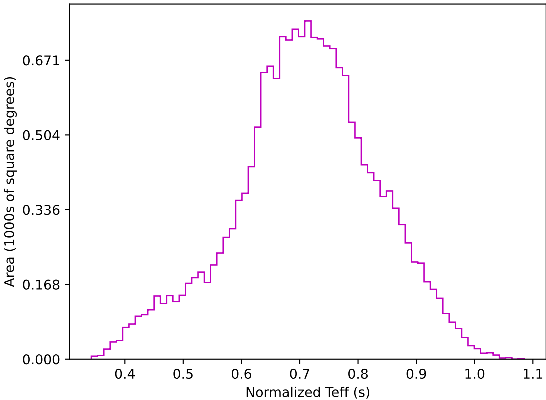
baseline_v3.5_10yrs WFD z band: Normalized Teff
