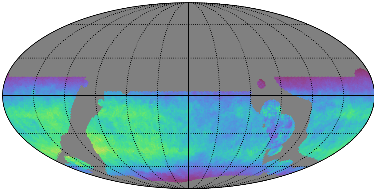
baseline_v3.5_10yrs WFD y band: Normalized Teff
