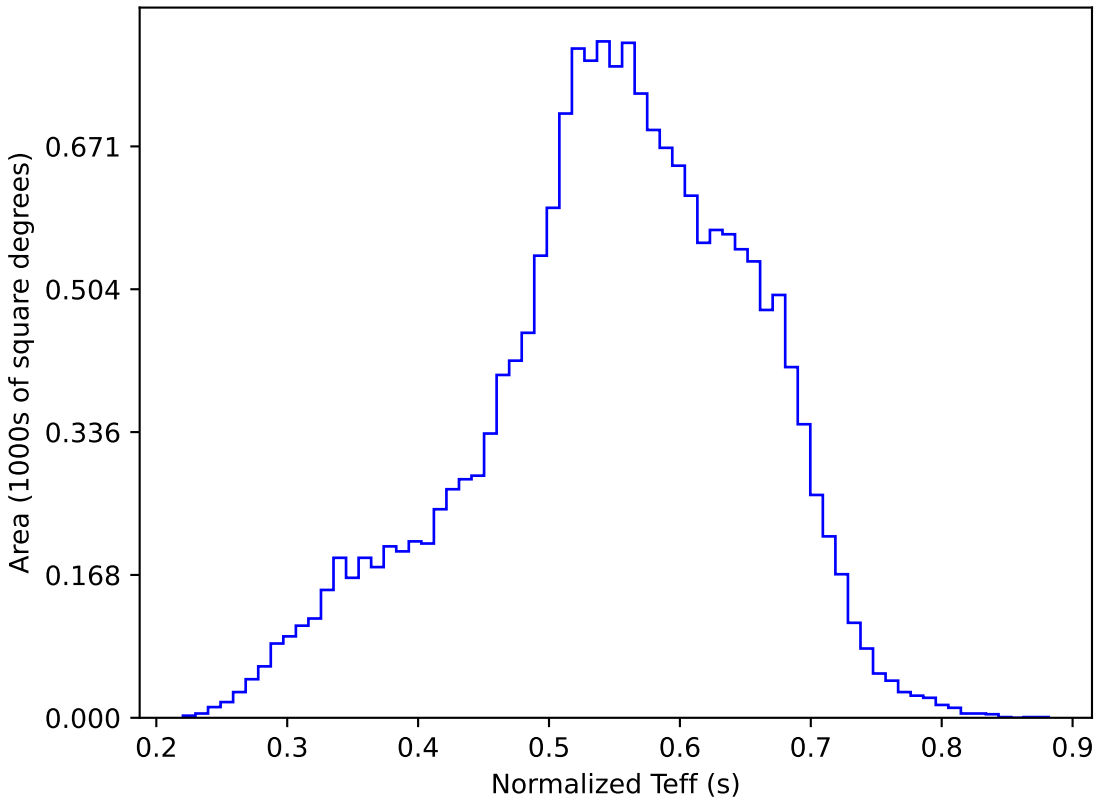
baseline_v3.5_10yrs WFD y band: Normalized Teff
