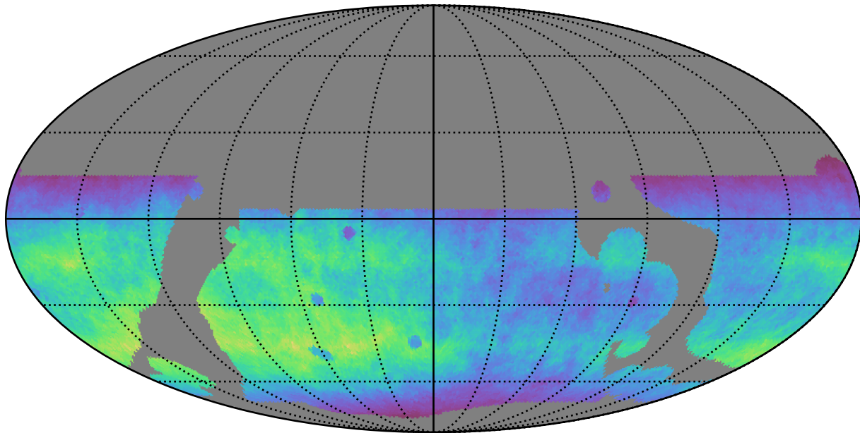
baseline_v3.5_10yrs WFD r band: Normalized Teff
