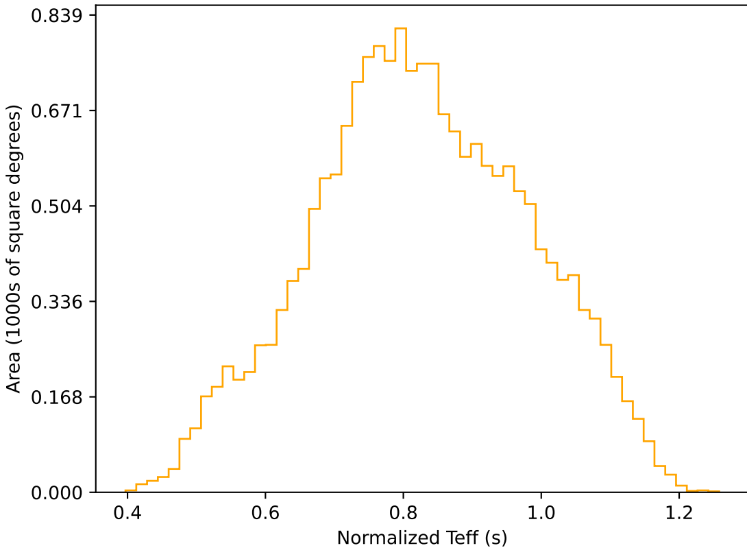
baseline_v3.5_10yrs WFD r band: Normalized Teff
