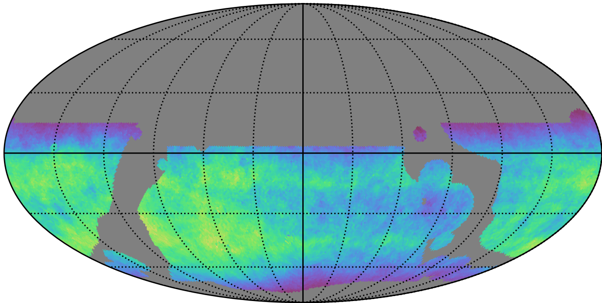
baseline_v3.5_10yrs WFD i band: Normalized Teff
