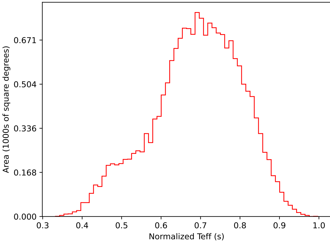
baseline_v3.5_10yrs WFD i band: Normalized Teff
