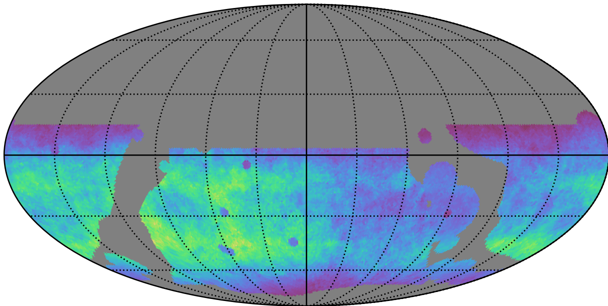
baseline_v3.5_10yrs WFD g band: Normalized Teff
