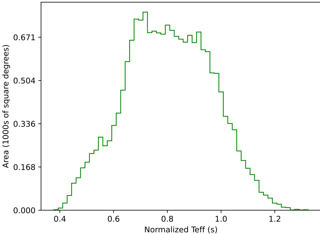
baseline_v3.5_10yrs WFD g band: Normalized Teff
