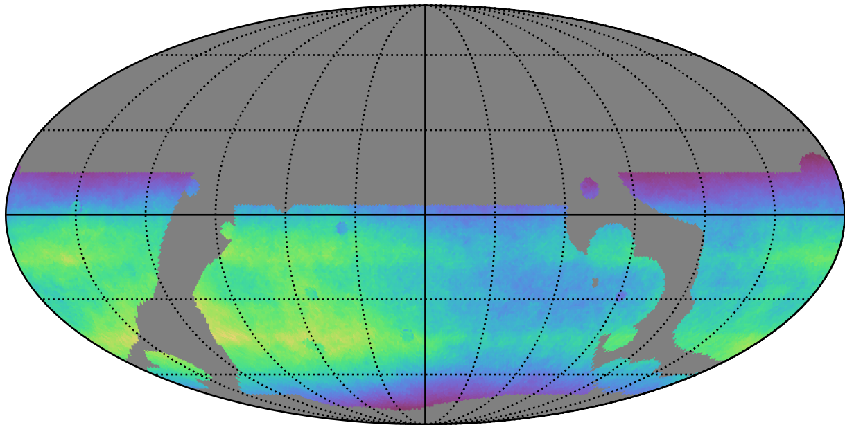
baseline_v3.5_10yrs WFD all bands: Normalized Teff
