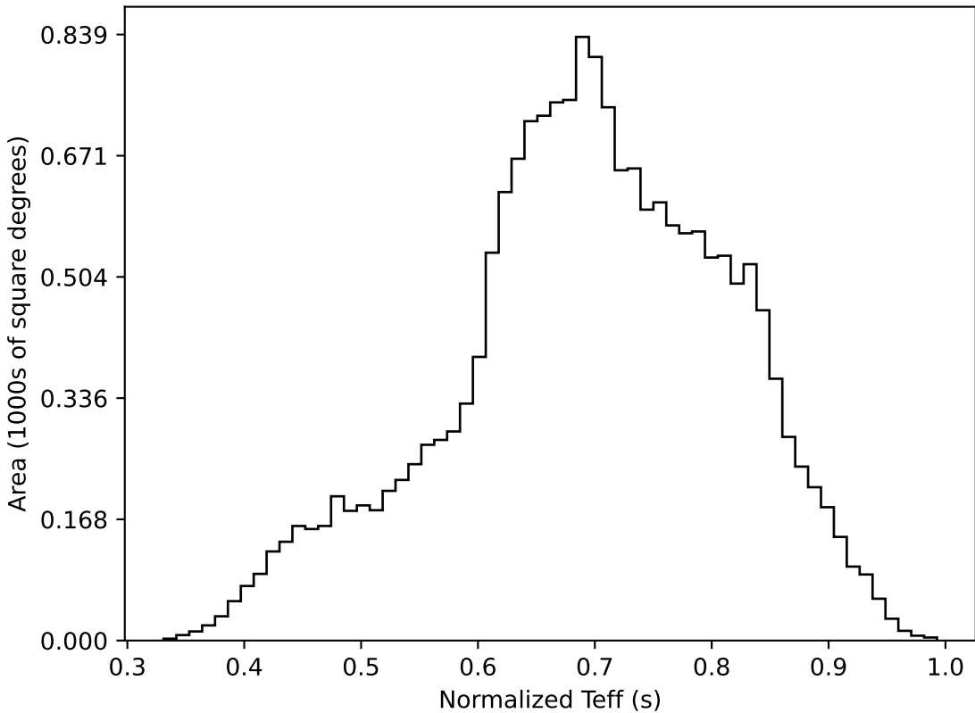
baseline_v3.5_10yrs WFD all bands: Normalized Teff
