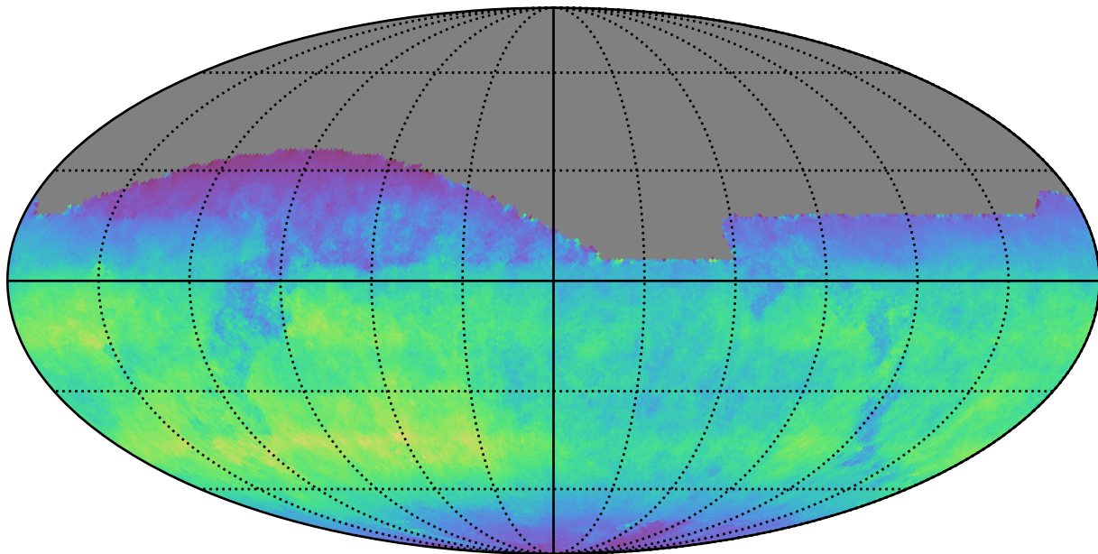
baseline_v3.5_10yrs All sky z band: Normalized Teff
