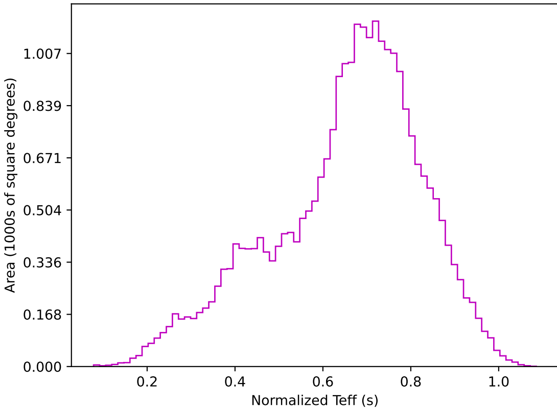
baseline_v3.5_10yrs All sky z band: Normalized Teff
