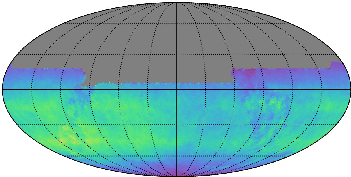
baseline_v3.5_10yrs All sky y band: Normalized Teff
