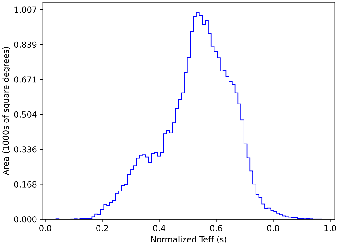
baseline_v3.5_10yrs All sky y band: Normalized Teff
