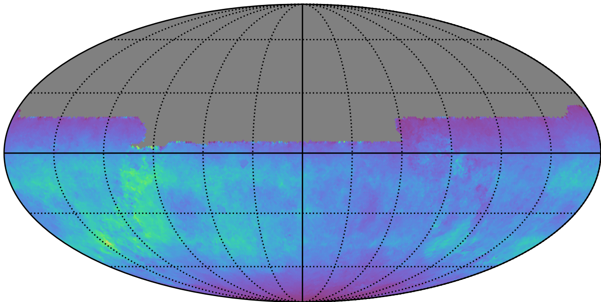
baseline_v3.5_10yrs All sky u band: Normalized Teff
