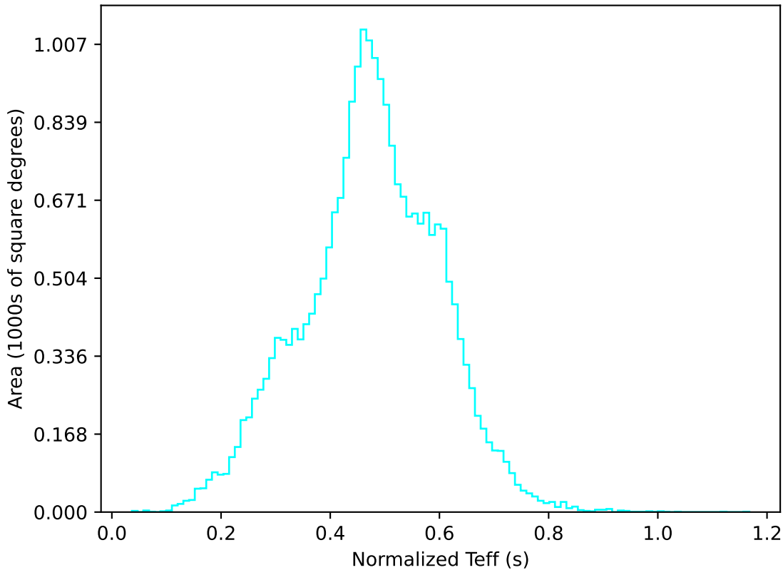
baseline_v3.5_10yrs All sky u band: Normalized Teff
