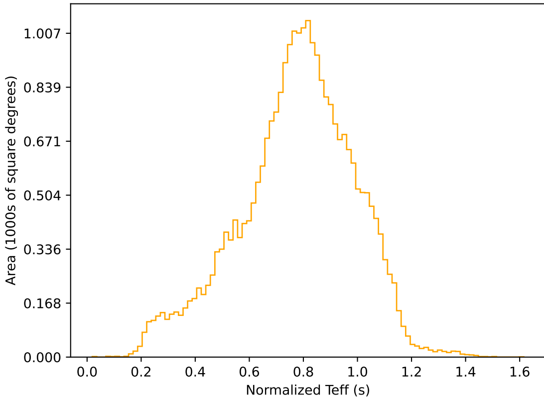
baseline_v3.5_10yrs All sky r band: Normalized Teff
