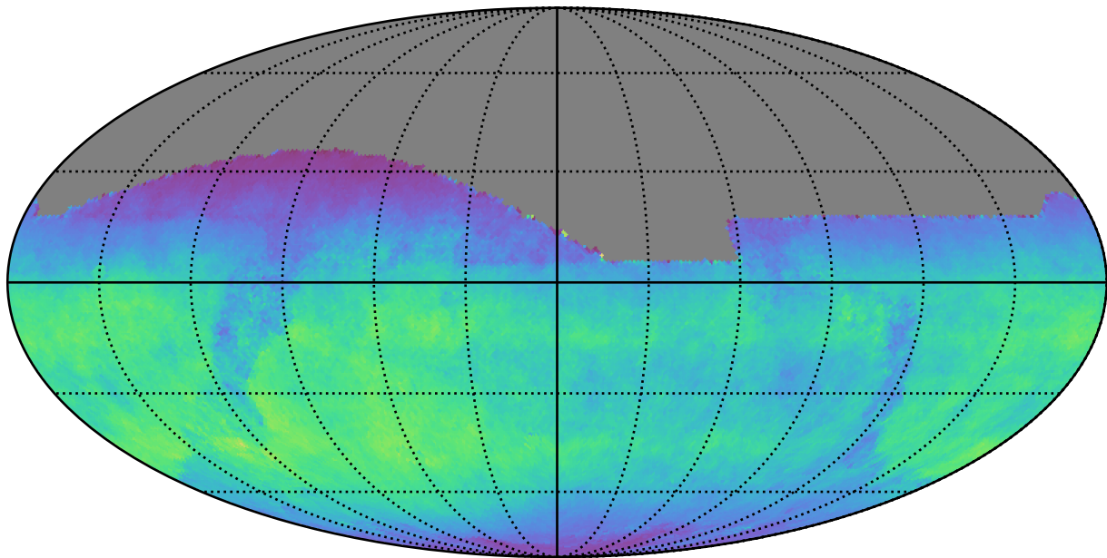
baseline_v3.5_10yrs All sky i band: Normalized Teff
