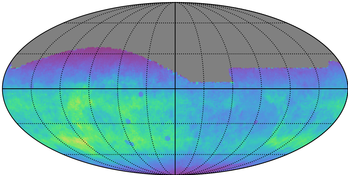
baseline_v3.5_10yrs All sky g band: Normalized Teff
