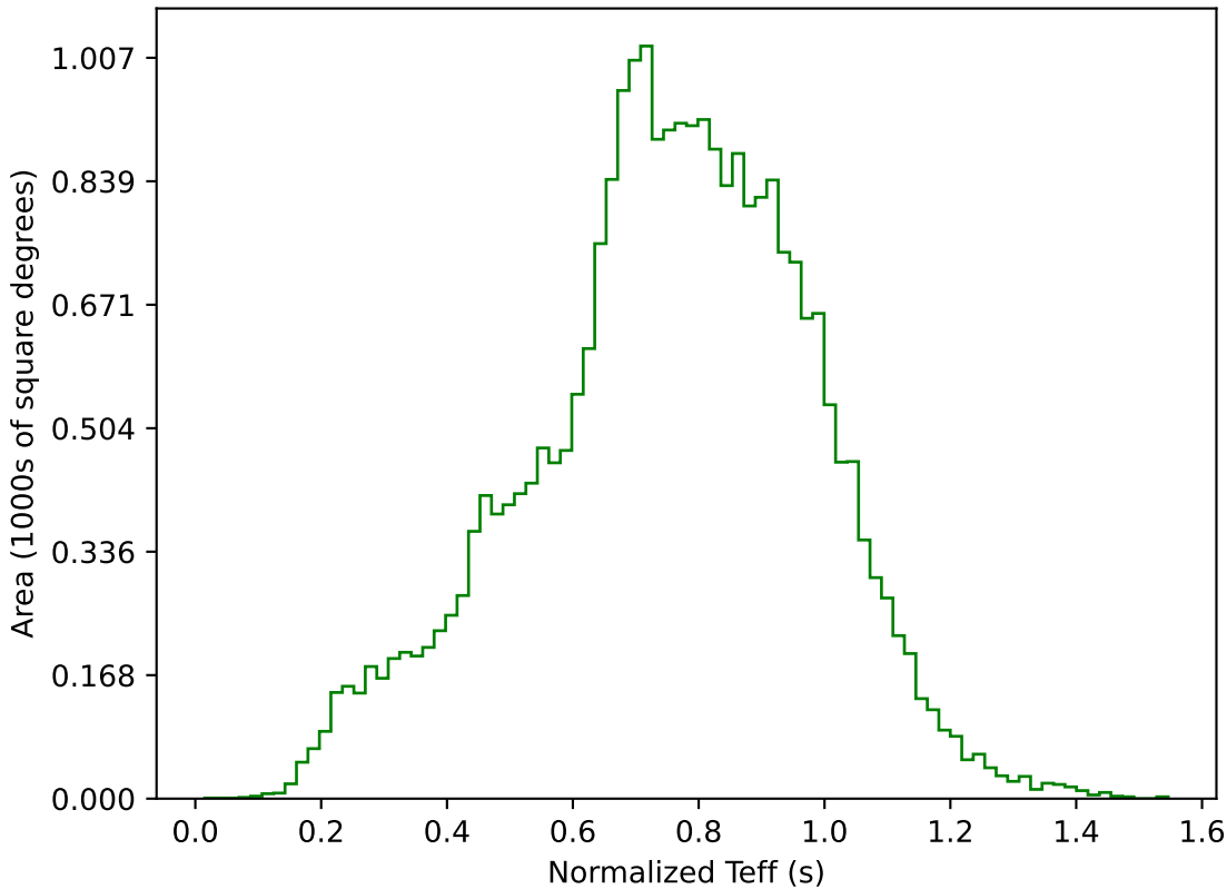
baseline_v3.5_10yrs All sky g band: Normalized Teff
