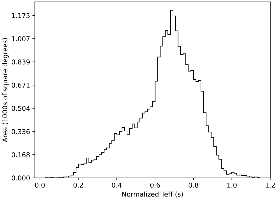
baseline_v3.5_10yrs All sky all bands: Normalized Teff
