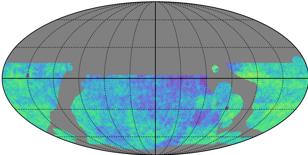
baseline_v3.5_10yrs WFD: Normalized Proper Motion Uncert @ 24.0
