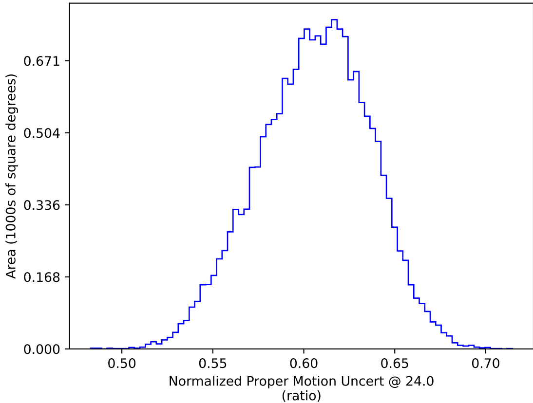
baseline_v3.5_10yrs WFD: Normalized Proper Motion Uncert @ 24.0
