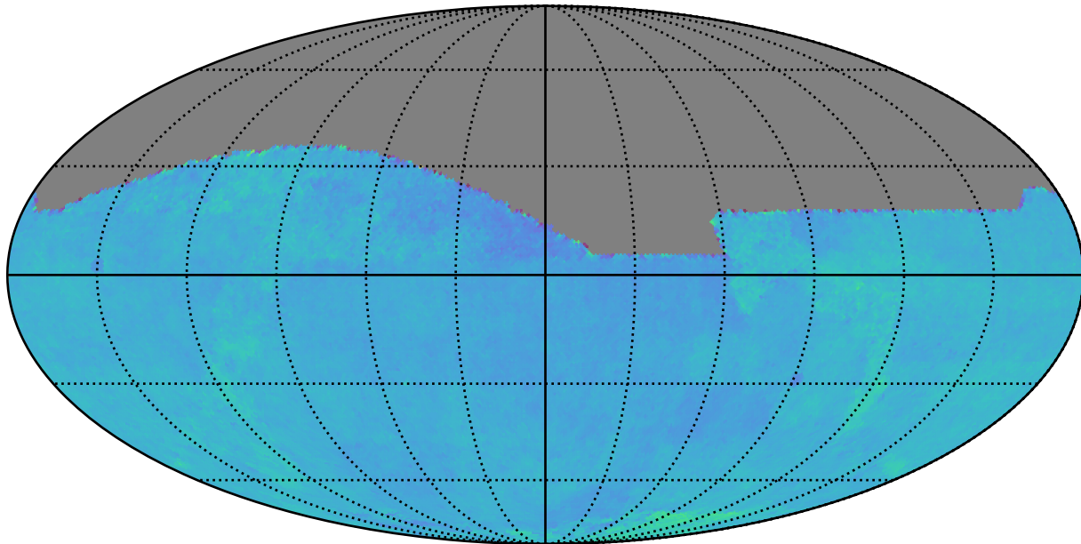
baseline_v3.5_10yrs All sky: Normalized Proper Motion Uncert @ 24.0
