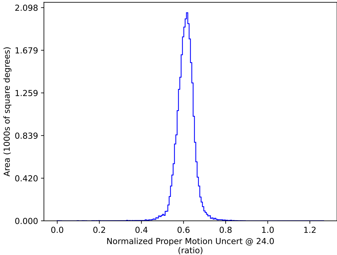
baseline_v3.5_10yrs All sky: Normalized Proper Motion Uncert @ 24.0
