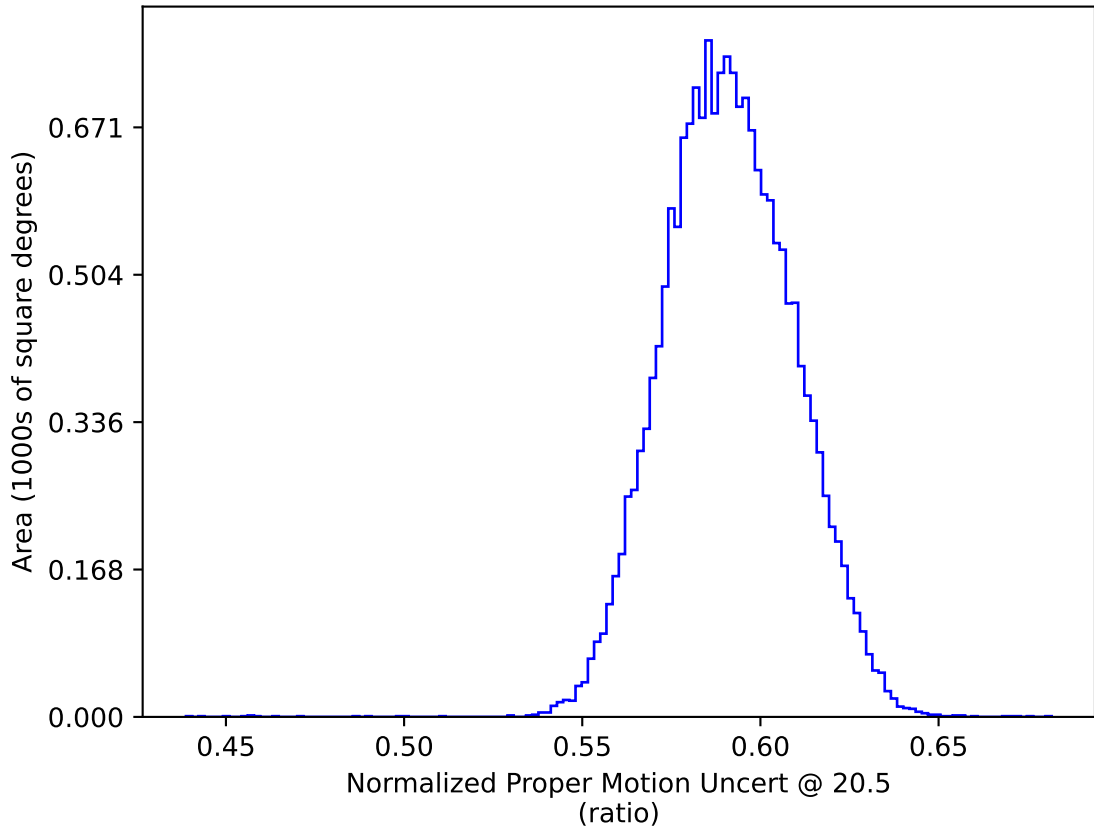
baseline_v3.5_10yrs WFD: Normalized Proper Motion Uncert @ 20.5
