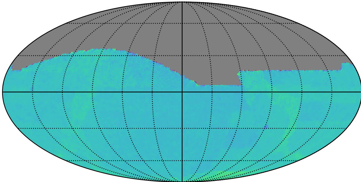
baseline_v3.5_10yrs All sky: Normalized Proper Motion Uncert @ 20.5
