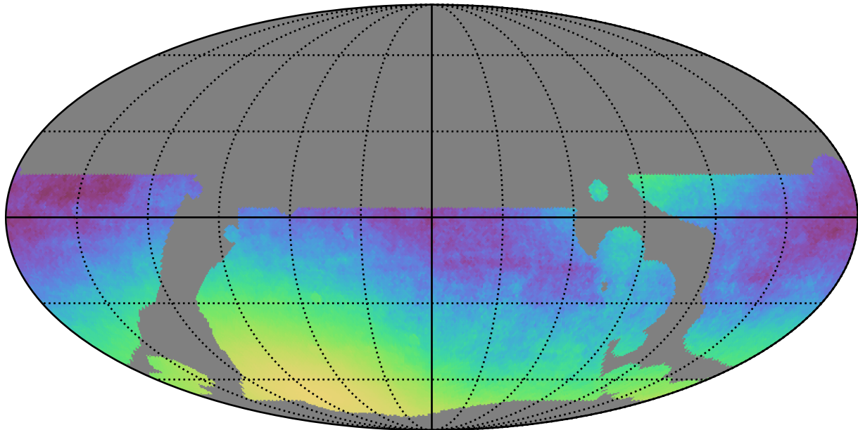
baseline_v3.5_10yrs WFD: Normalized Parallax Uncert @ 24.0
