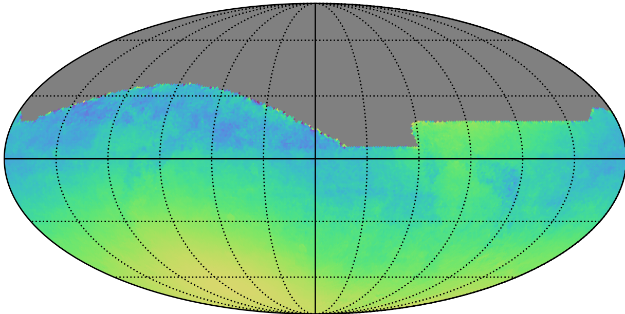
baseline_v3.5_10yrs All sky: Normalized Parallax Uncert @ 24.0
