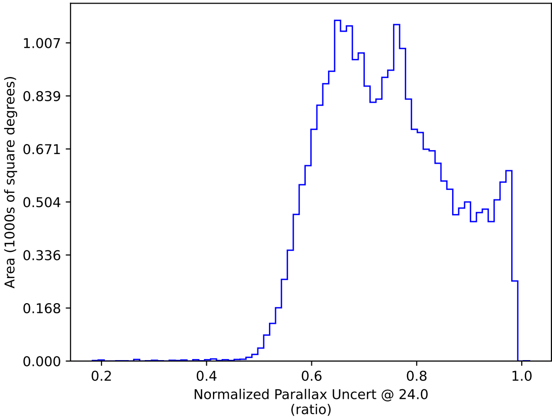
baseline_v3.5_10yrs All sky: Normalized Parallax Uncert @ 24.0
