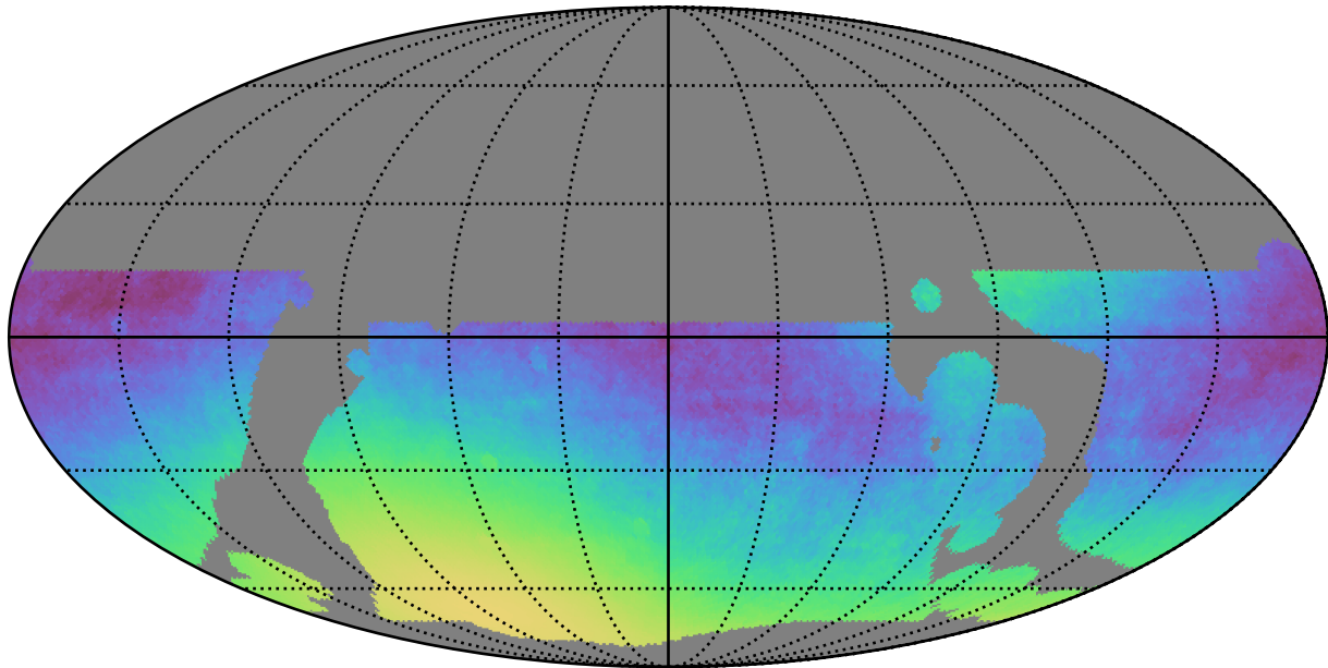
baseline_v3.5_10yrs WFD: Normalized Parallax Uncert @ 22.4
