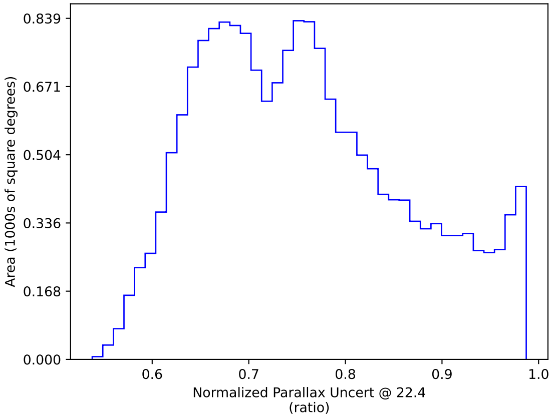
baseline_v3.5_10yrs WFD: Normalized Parallax Uncert @ 22.4
