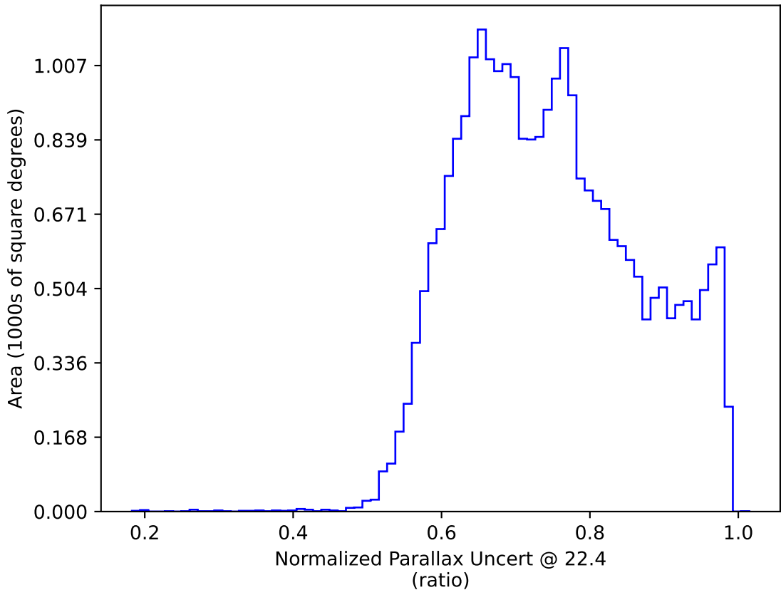
baseline_v3.5_10yrs All sky: Normalized Parallax Uncert @ 22.4
