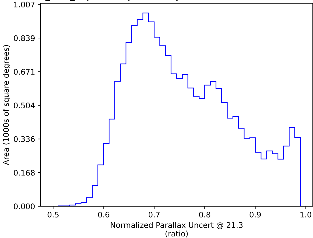
baseline_v3.5_10yrs WFD y band only: Normalized Parallax Uncert @ 21.3
