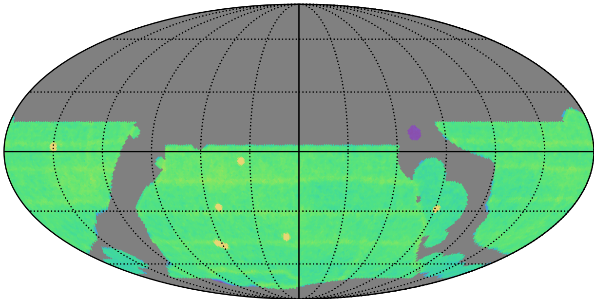
baseline_v3.5_10yrs WFD all bands: N Unique Nights
