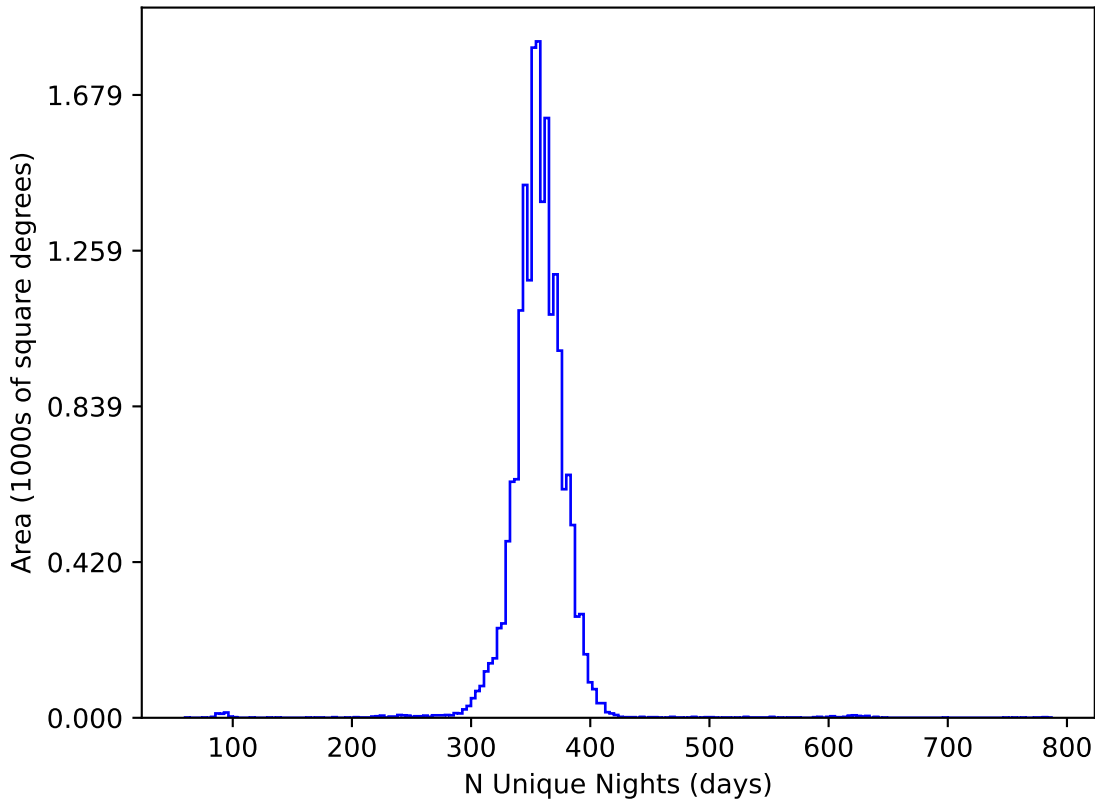
baseline_v3.5_10yrs WFD all bands: N Unique Nights
