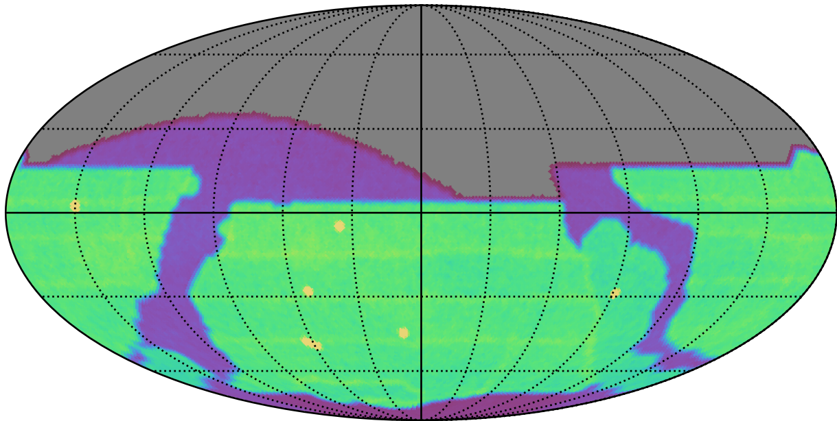
baseline_v3.5_10yrs All sky all bands: N Unique Nights
