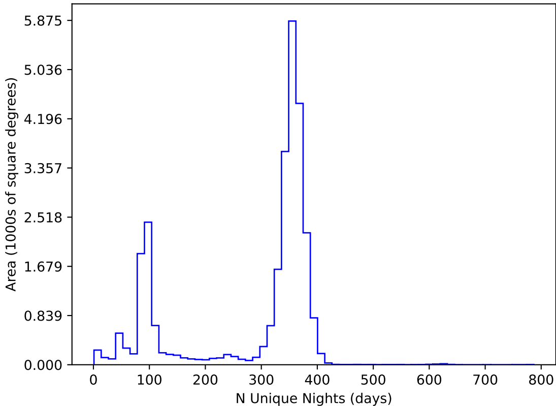
baseline_v3.5_10yrs All sky all bands: N Unique Nights
