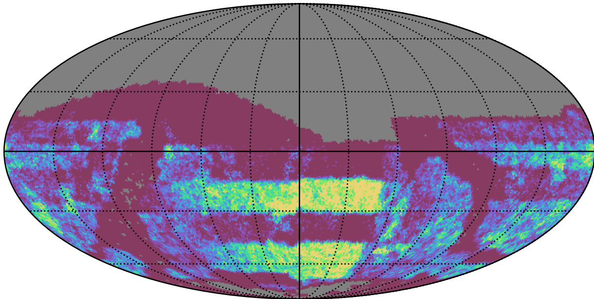
baseline_v3.5_10yrs Yr 3-4 z band: NVisits
