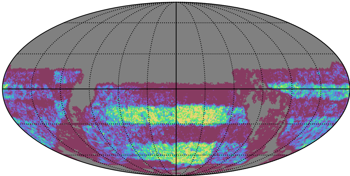
baseline_v3.5_10yrs Yr 3-4 y band: NVisits
