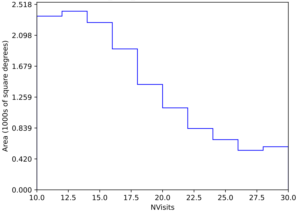
baseline_v3.5_10yrs Yr 3-4 y band: NVisits
